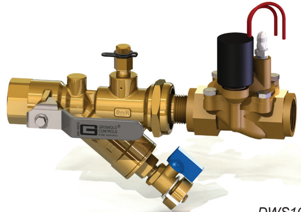
DWS100.IS DWS valve with a combination ball valve, strainer, and union valve
