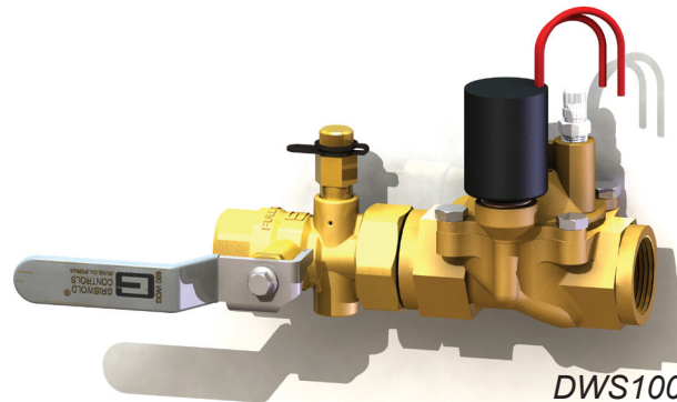
DWS100.IS DWS valve with a combination ball valve, strainer, and union valve
