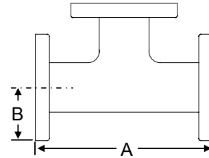
Flanged Tee
