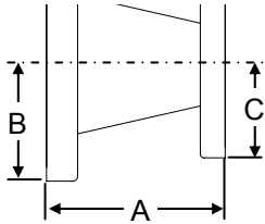
Flange Reducer
