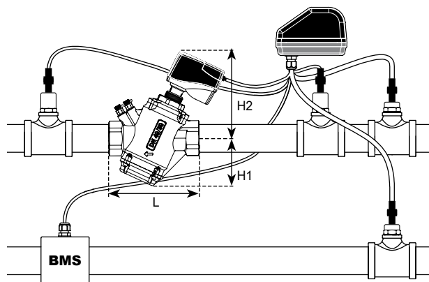
Griswold Controls FIT-G.3 with FH actuator, Intelligent Interface and sensor kit
